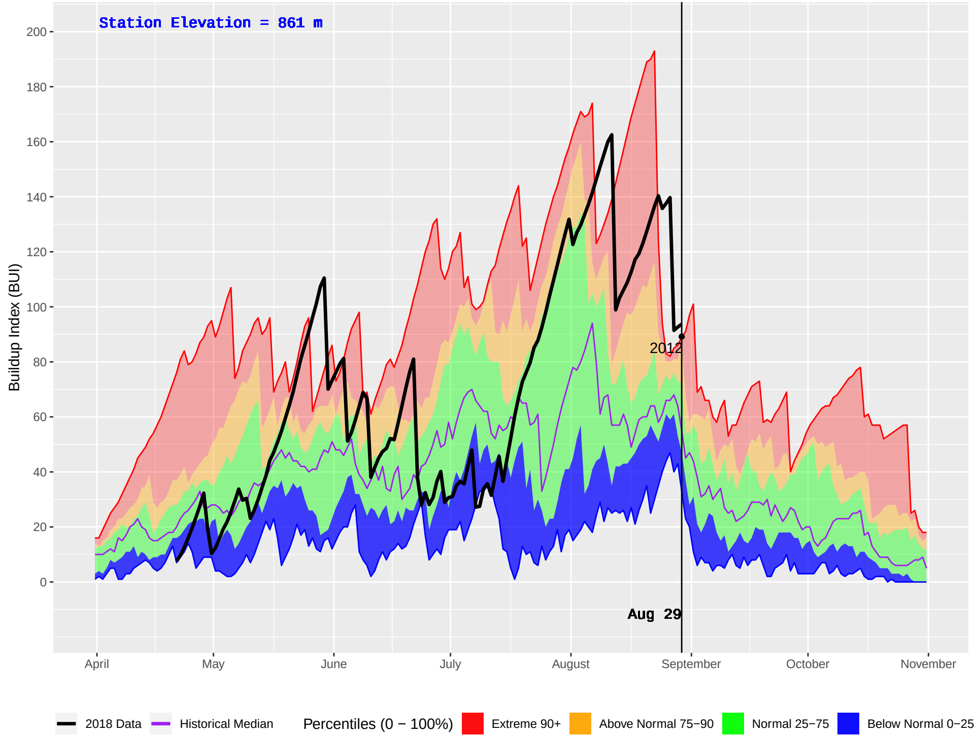
BLAEBERRY (866) : Historical (2004–2016) and Current (2018) Daily Buildup Index (BUI)
